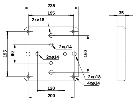
Fig. 48 Base plate
