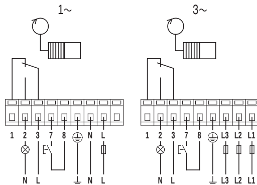
Fig. 36 Operating indication
