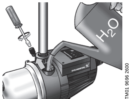
Fig. 14 Priming the pump
